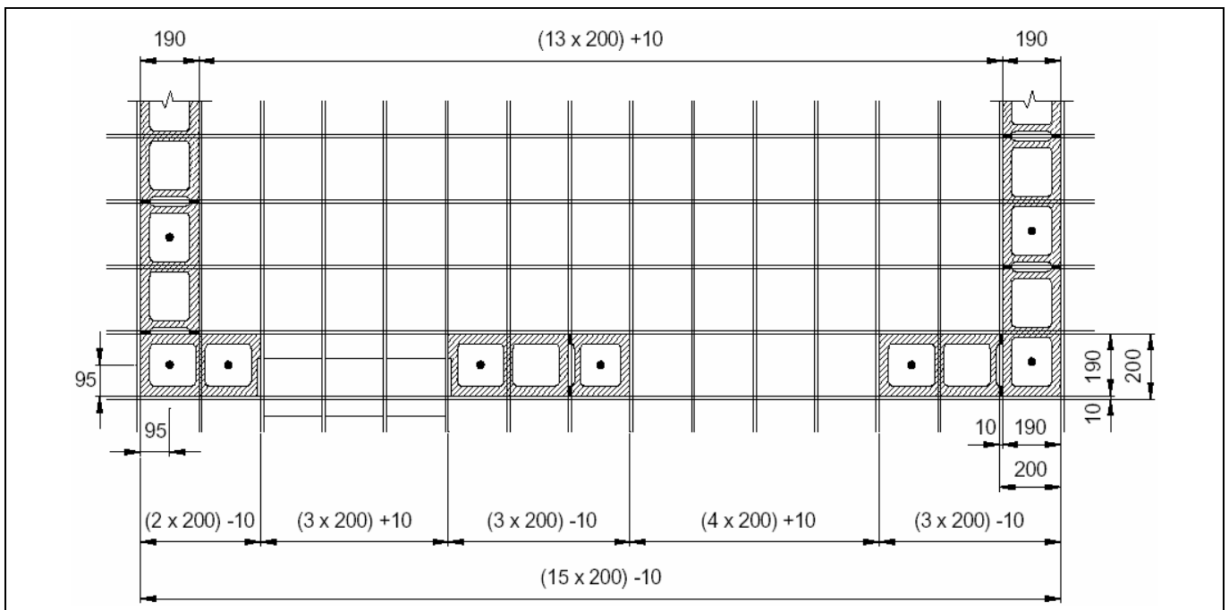
Figure 1: Planning on the standards concrete masonry grid.
